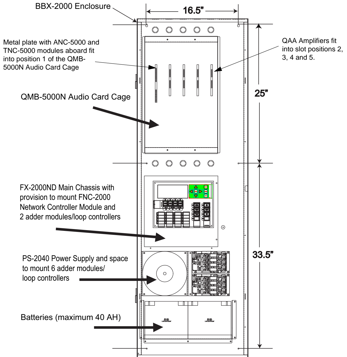
Figure 1: BBX-2000 Enclosure with the Integrated Fire and Audio System
