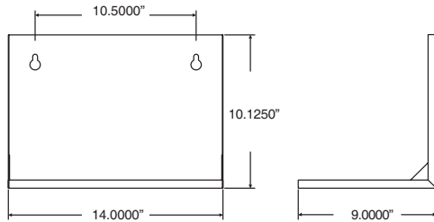
MPS30 - MLS series battery unit, over 200W (Type 3 cabinet)
