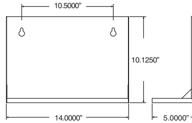
MPS20 - MLS series battery unit, 200W and under (Type 3 cabinet)
