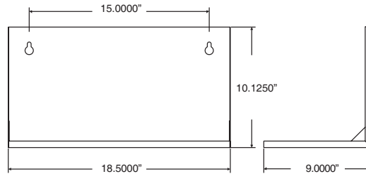
MPS40 - MLS series battery unit (Type 4 cabinet)
