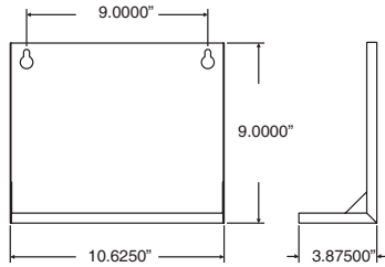
MPS10 - MLS series battery unit (Type 2 cabinet)
