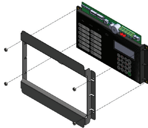
Some enclosures require the installation of the CH-1074B, included with the RAM-3318-LCD
