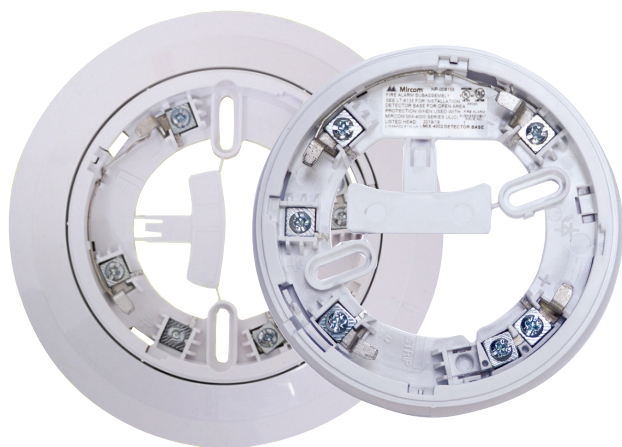
MIX-4001 / MIX-4002
