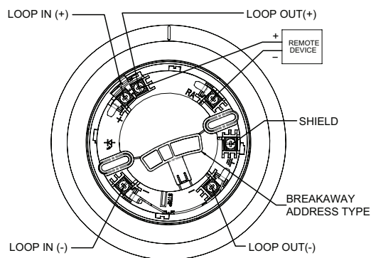
DETECTOR WIRING
