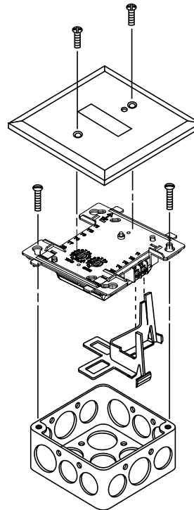
FIGURE 2A. MODULE MOUNTING WITH BARRIER:
