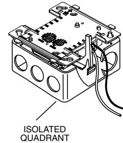
FIGURE 2A. MODULE MOUNTING WITH BARRIER:
