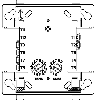
FIGURE 1. CONTROLS AND INDICATORS:
