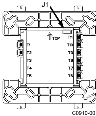
FIGURE 1B: JUMPER LOCATION
