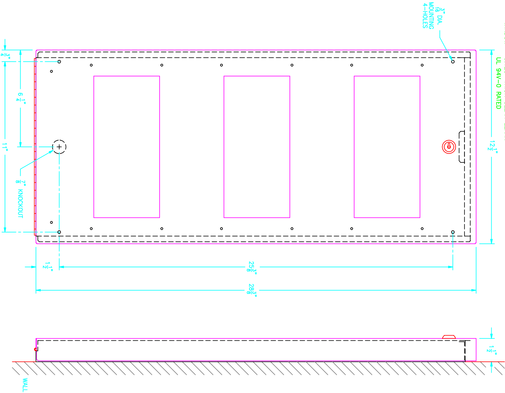
FRONT VIEW
