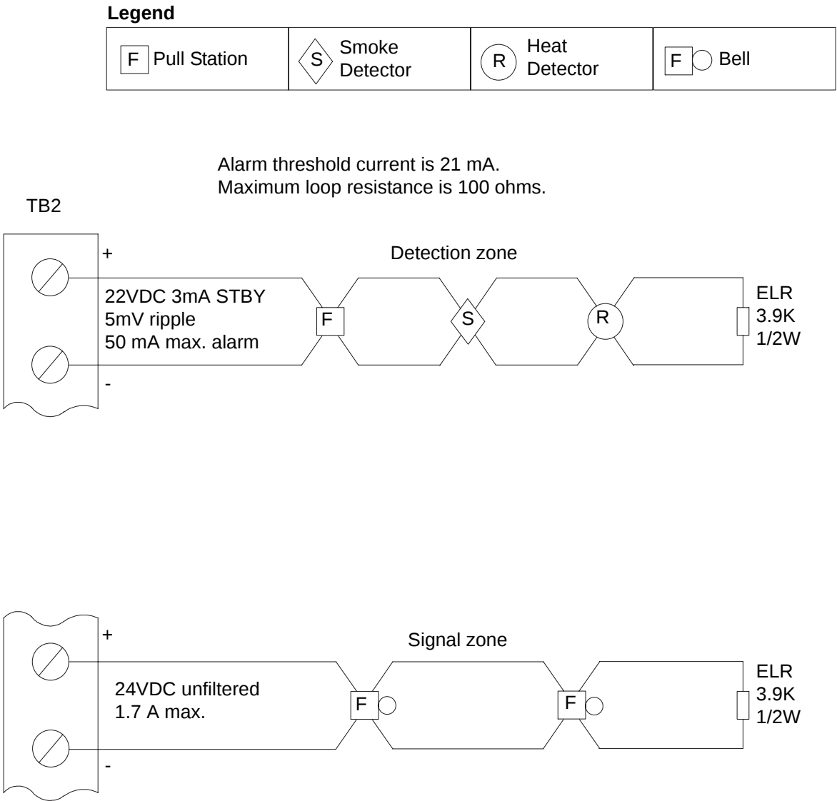
Figure 3: Detection and Signal Wiring
