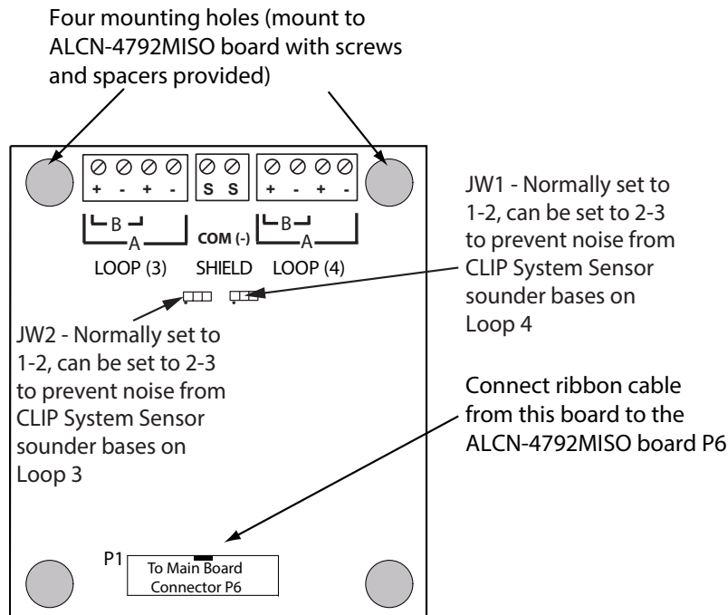
Figure 2: ALCN-792D Daughter Board
