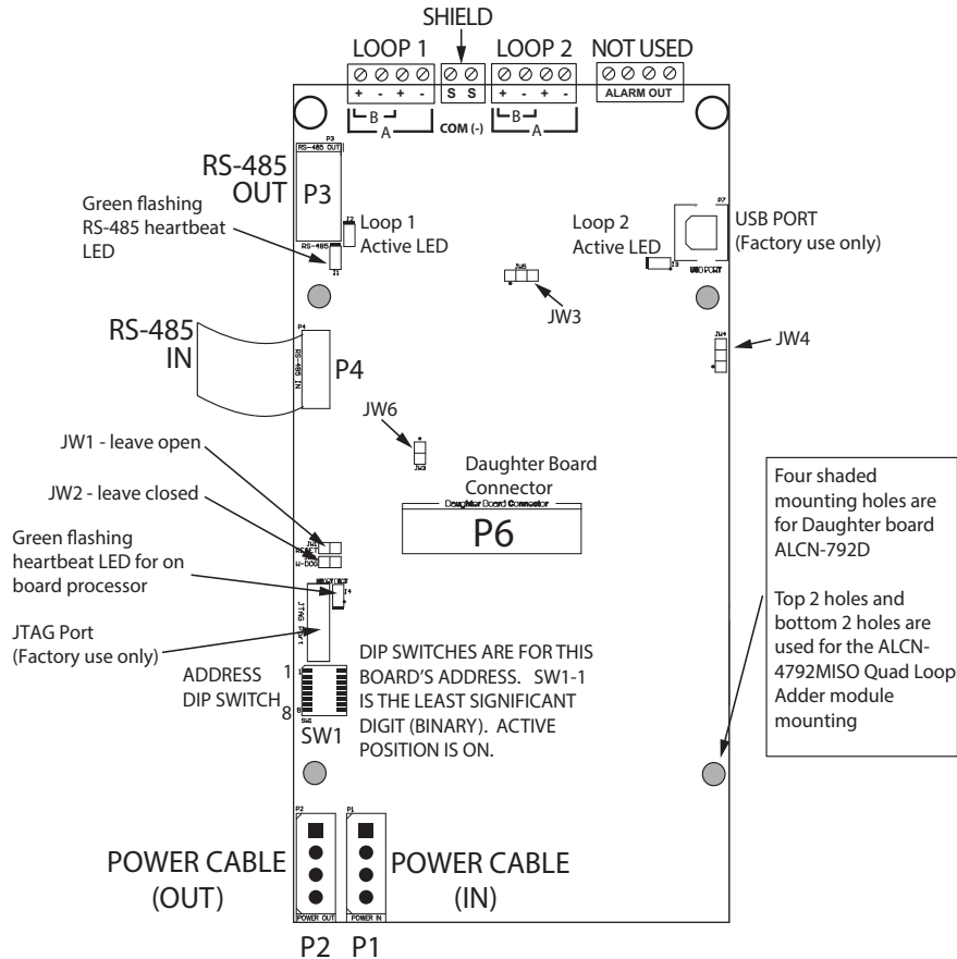
Figure 1: ALCN-4792MISO Isolated Quad Loop Adder Module
