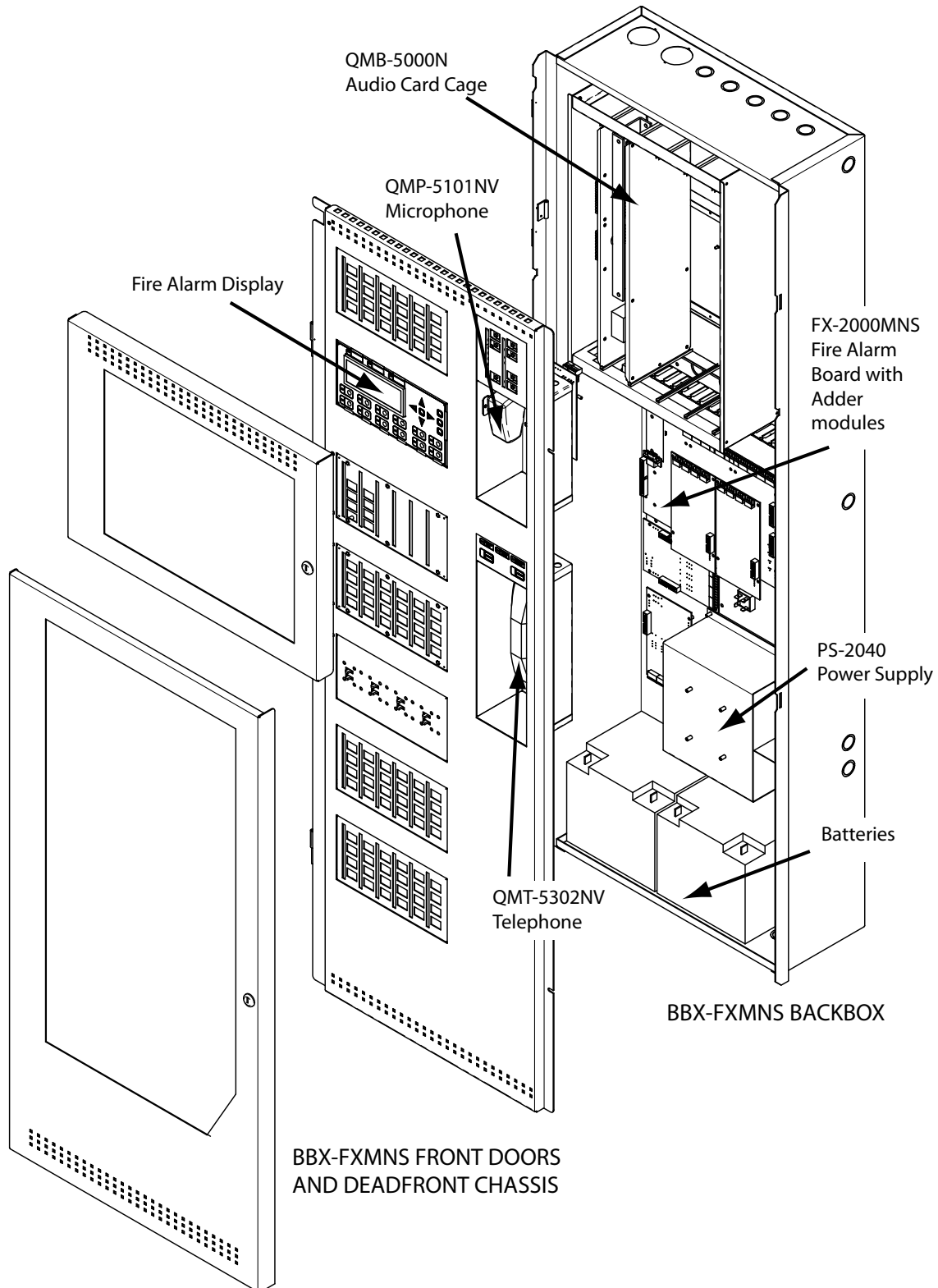
Figure 2: Expanded View of the BBX-FXMNS Enclosure
