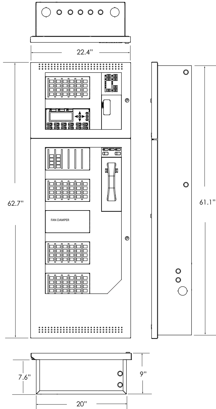
Figure 1: BBX-FXMNS Enclosure with Dimensions
