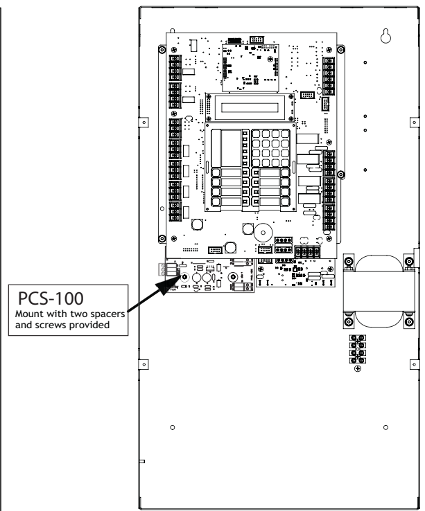
FX-351 Panels
