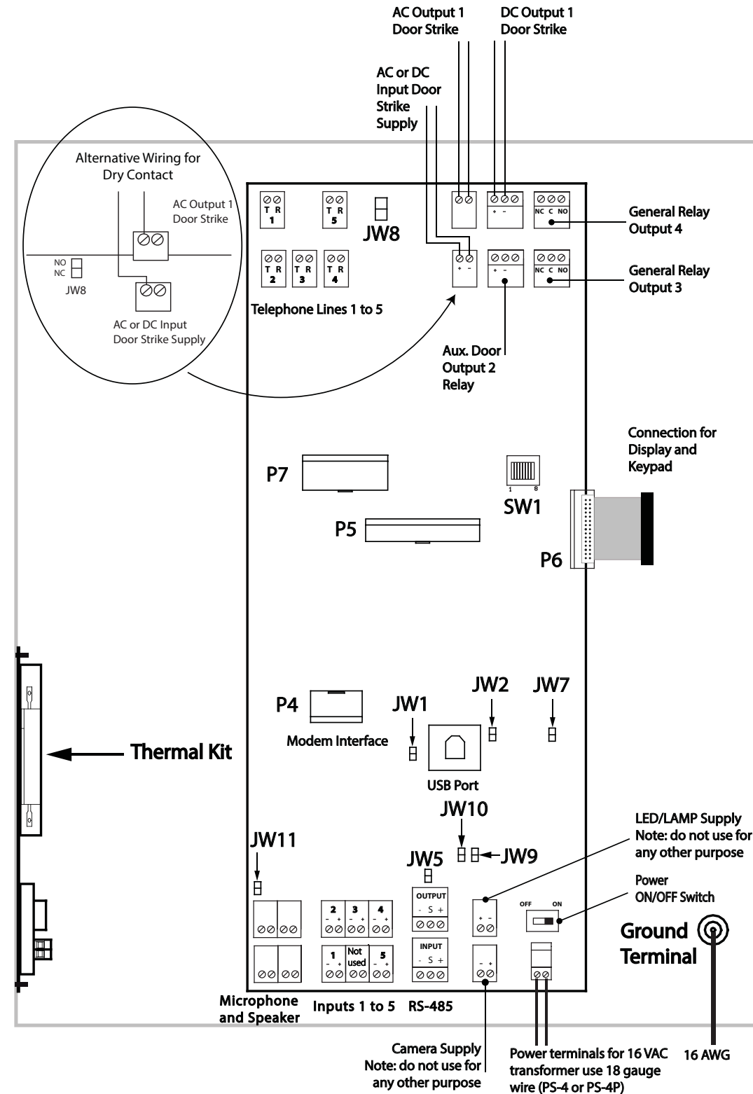
TELEPHONE ACCESS BOARD WIRING FOR TX3 MODELS ENDING IN -C
