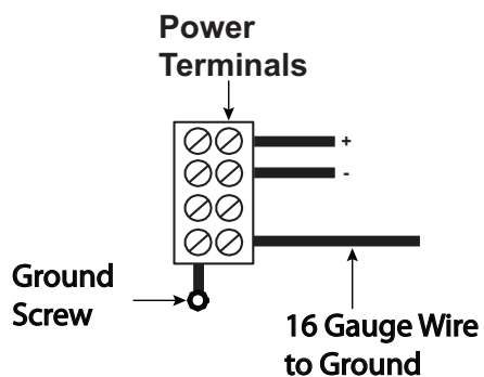
Figure 2. Grounding the 22" Touch Screen
