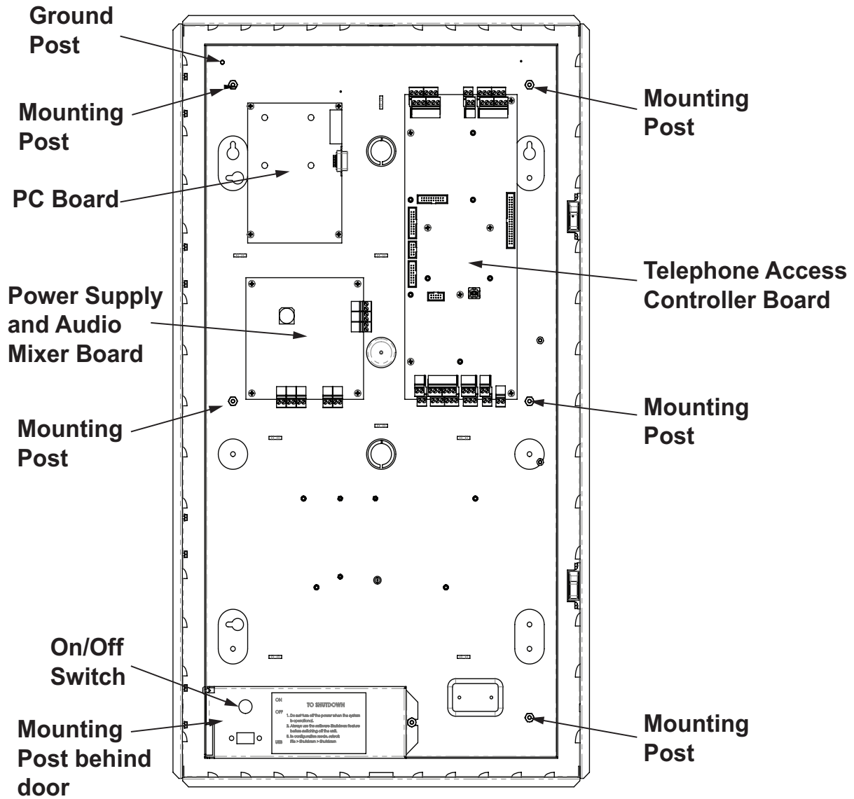
Figure 1 Inner chassis mounted in enclosure
