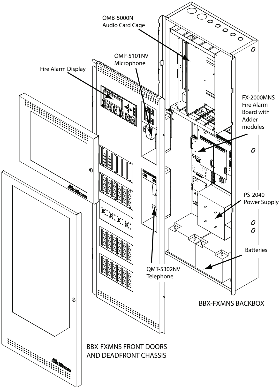
Figure 2: Expanded View of the BBX-FXMNSRG Enclosure
