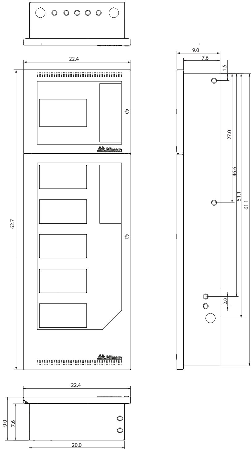
Figure 1: BBX-FXMNSRG Enclosure with Dimensions
