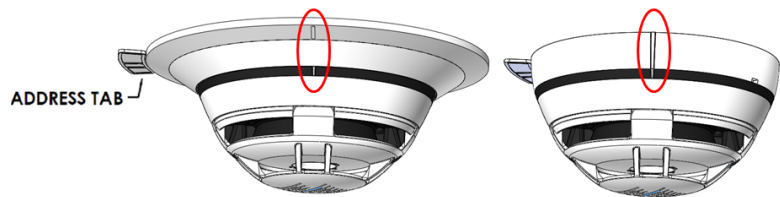
FIGURE 4: ALIGNMENT MARKS
