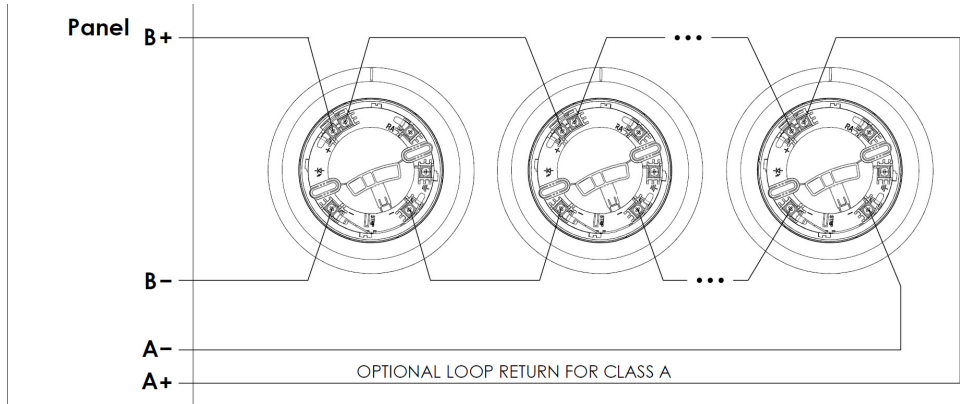
FIGURE 3: LOOP WIRING
