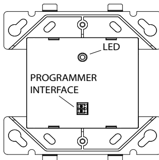
FIGURE 1: MODULE FRONT
