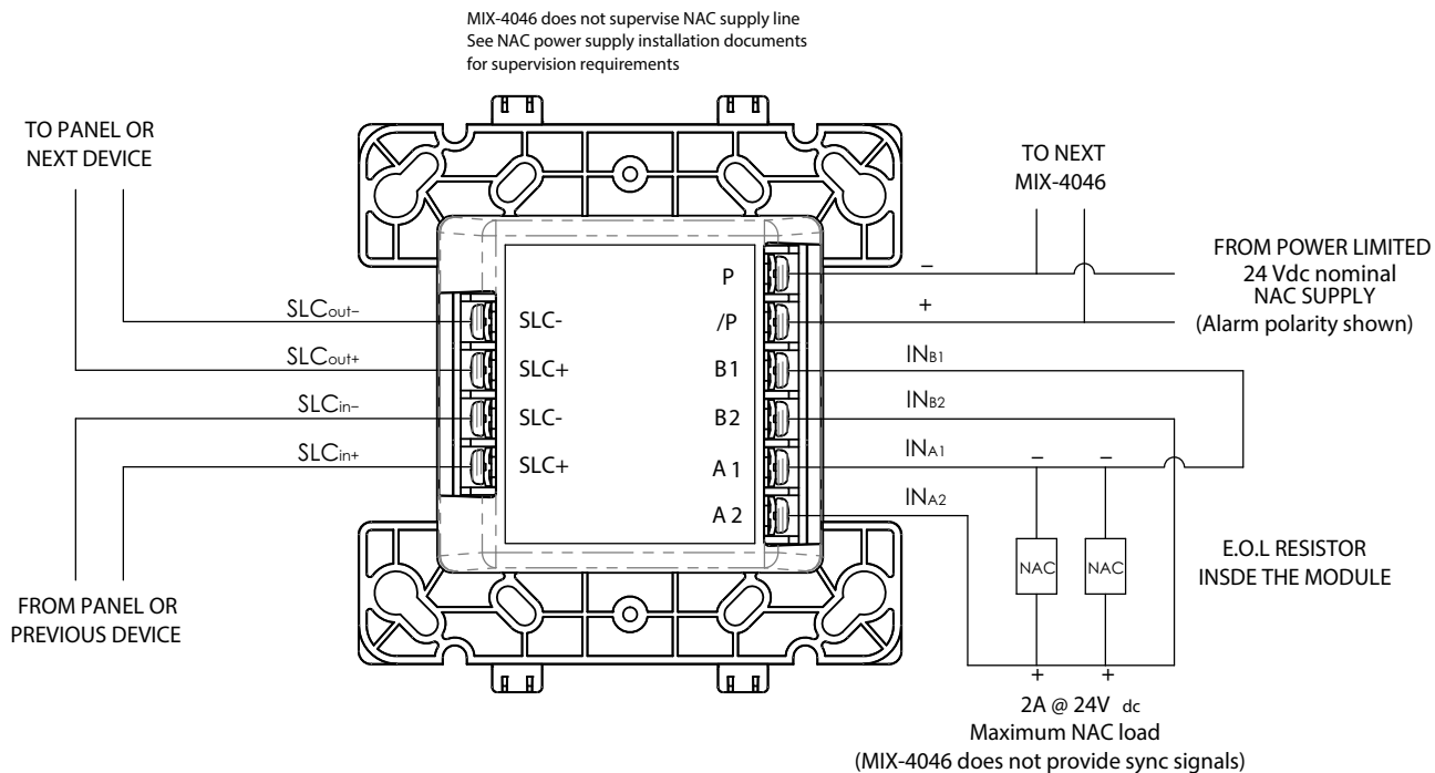
FIGURE 5: SAMPLE CLASS A NAC WIRING
