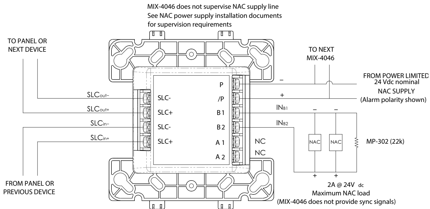
FIGURE 6: SAMPLE CLASS B NAC WIRING
