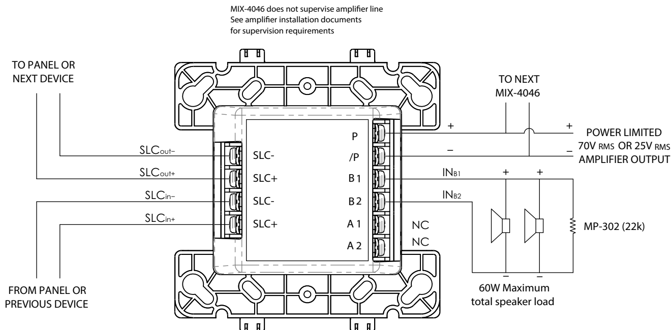
FIGURE 8: SAMPLE CLASS B SPEAKER WIRING
