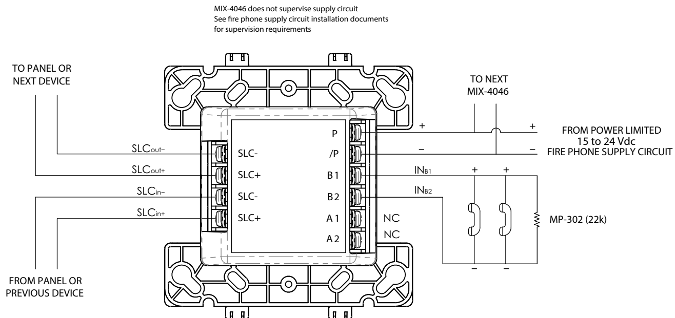
FIGURE 4: SAMPLE CLASS B FIRE PHONE WIRING:
