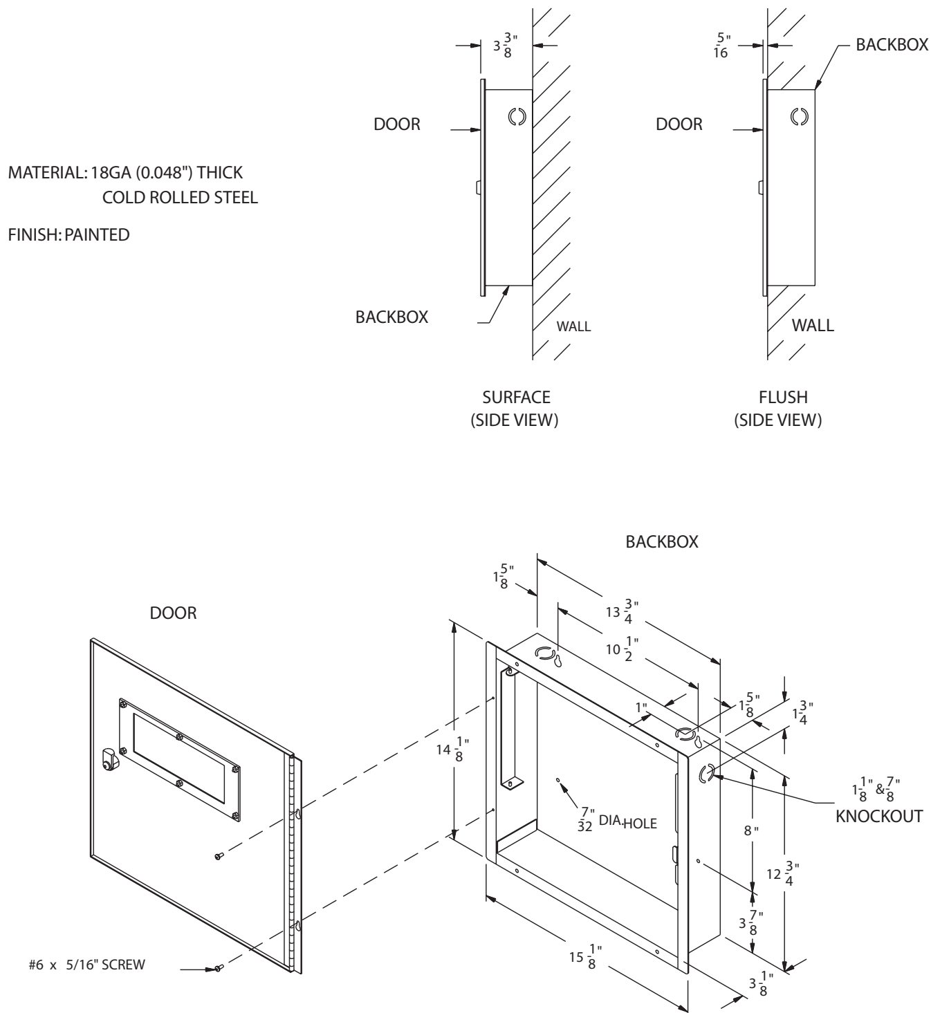
Figure 1: FA-201, 202, and 204 Enclosure Installation and Dimensions
