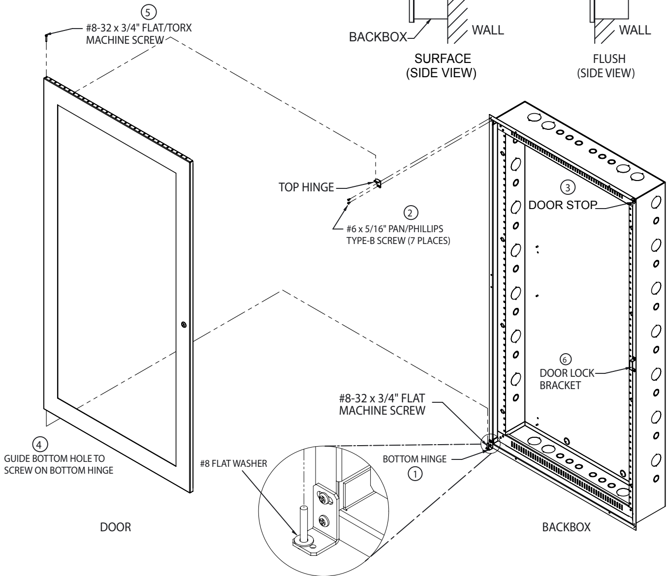
Lobby Control Center Steel Door (Model: DOX-5014M) Installation Instruction and Dimensions
