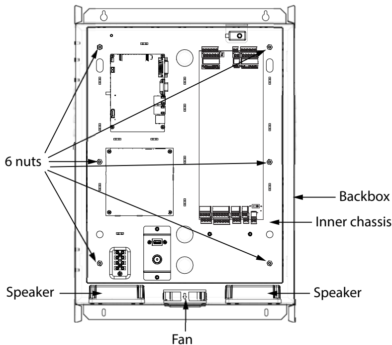
Figure 1 Inner chassis
