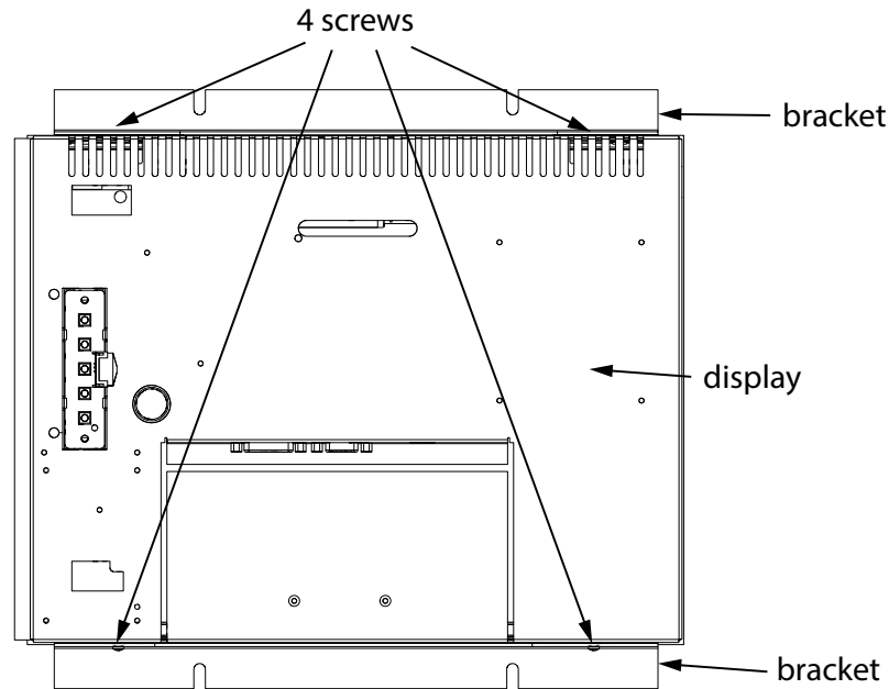
Figure 1 Display assembly
