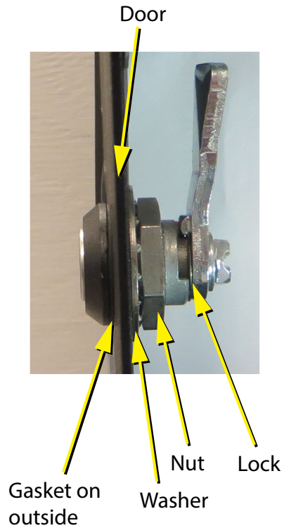
Figure 2 Lockset
