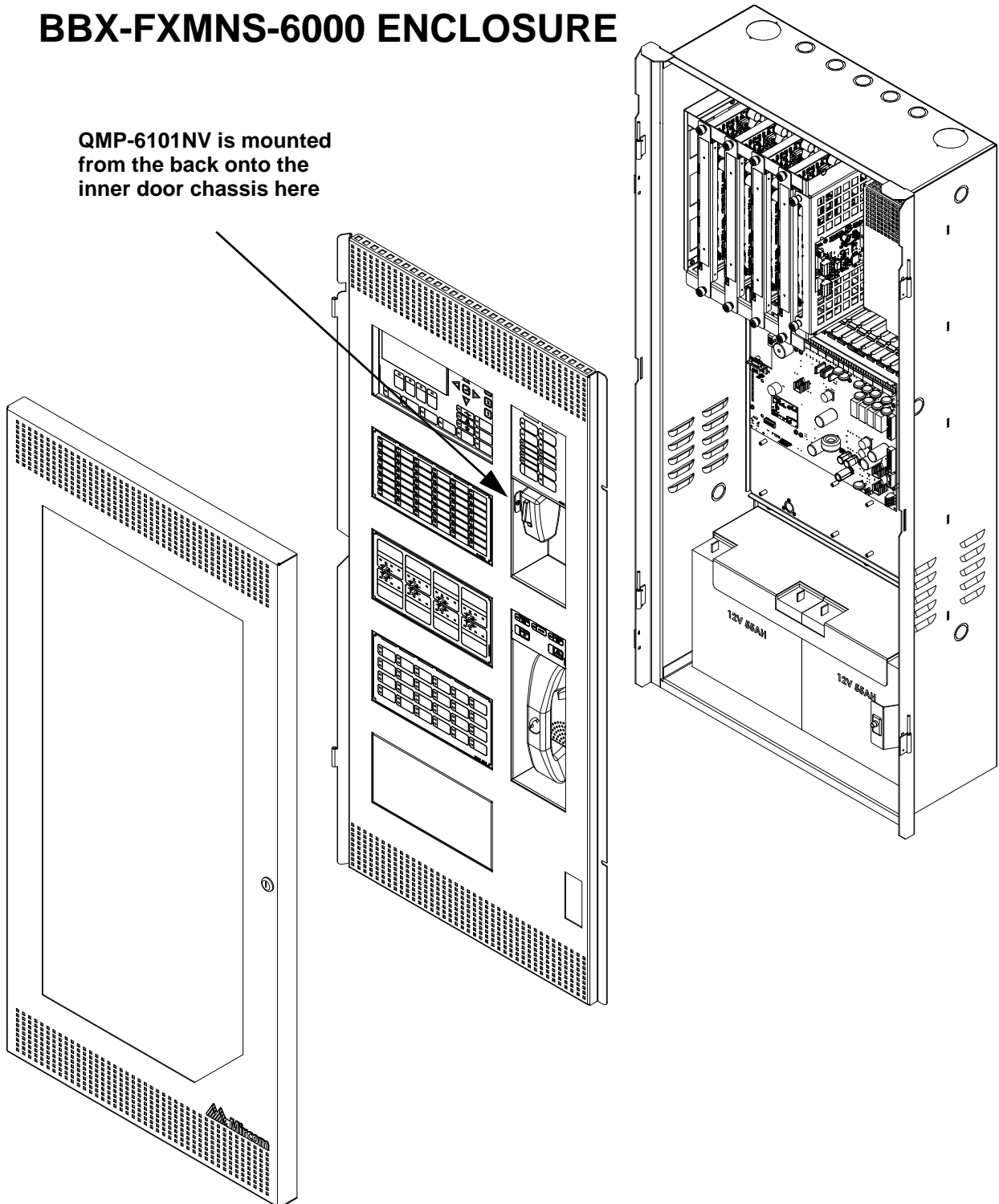
Figure 2 Mounting the QMP-6101NV into the BBX-FXMNS-6000 Enclosure
