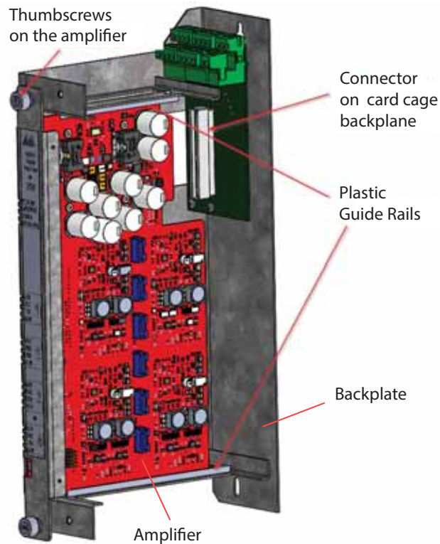
Figure 2 Partial view of Amplifier Connected to Card Cage Backplane
