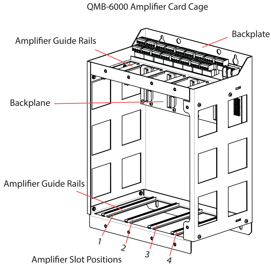
Figure 1 QMB-6000 Amplifier Card Cage
