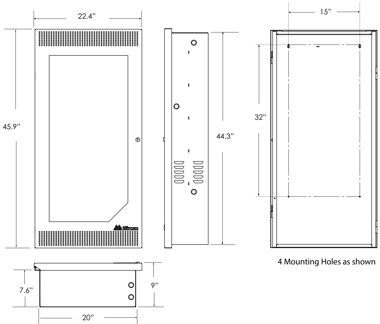
Figure 1: BBX-FXMNS-6000 Dimensions, Mounting Holes and Knockouts for Installation
