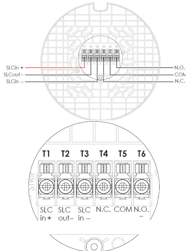
FIGURE 4: WIRING TABS
