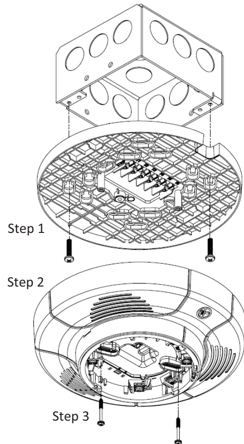
FIGURE 6: MOUNTING DIAGRAM
