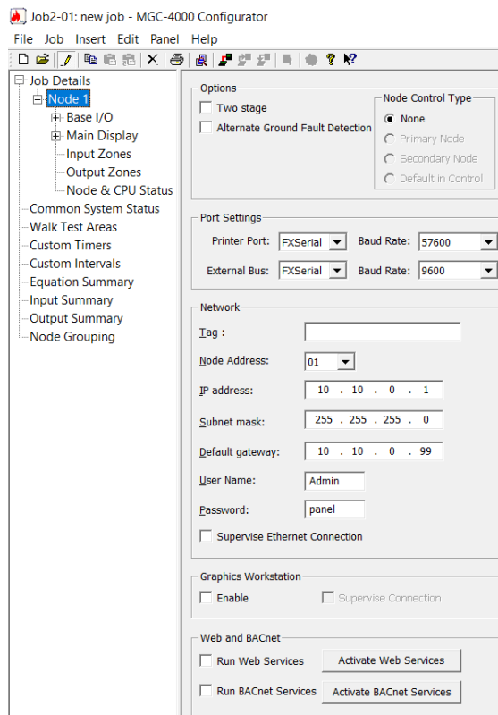
Figure 5 Network Node Details
