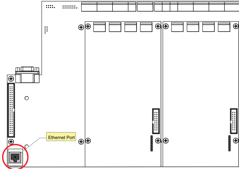
Figure 1 FleX-Net™ FX-4000 Main Board Ethernet Port (P7) Location
