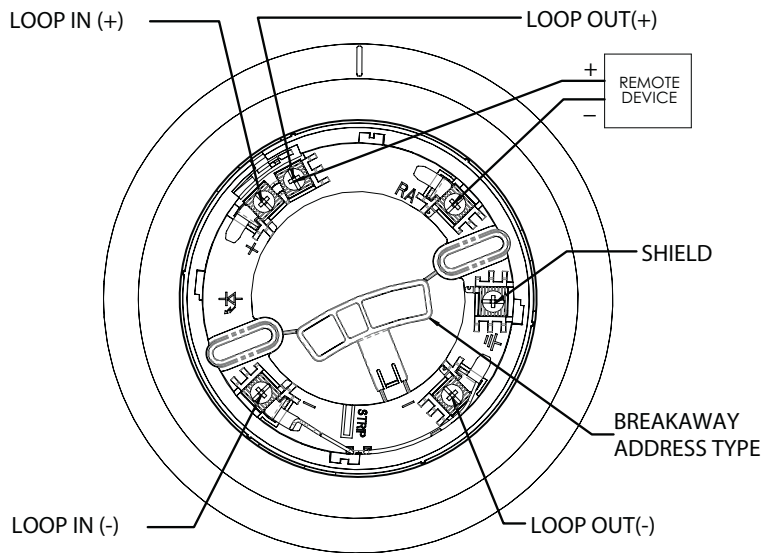
FIGURE 2: DETECTOR WIRING
