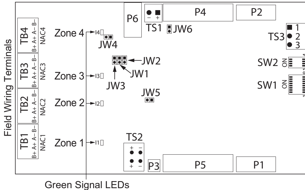
Figure 2 Signal Adder Module SGM-1004S
