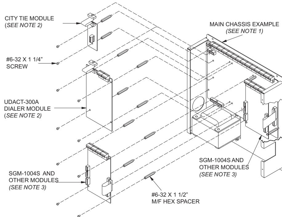
Figure 1 Module Mounting Locations
