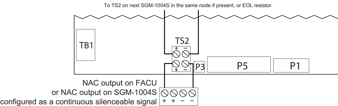
Figure 4 Audible Signal Silence Mode Wiring
