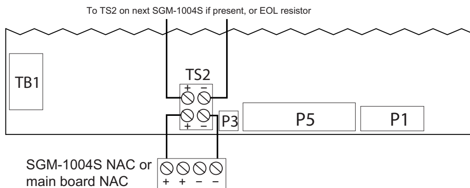
Figure 5 External Sync Mode Wiring
