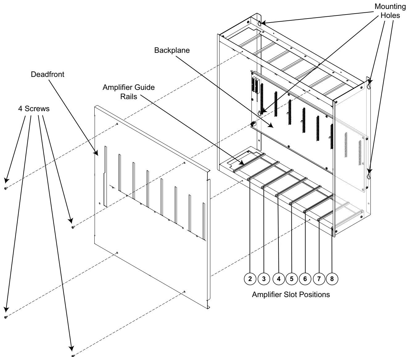
Figure 1 QMB-5000B Audio Motherboard and Card Cage and Mounting Hole Locations
