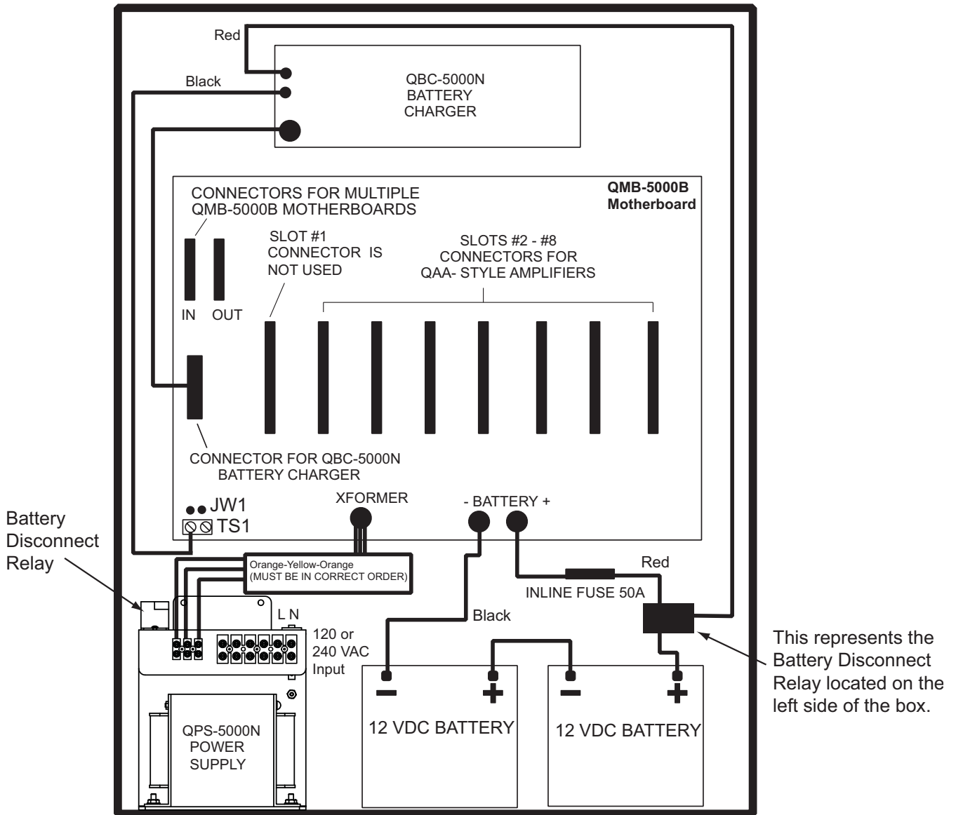
Figure 2 Placement of QMB-5000B Audio Motherboard in QBB-5001R Expansion Audio Cabinet
