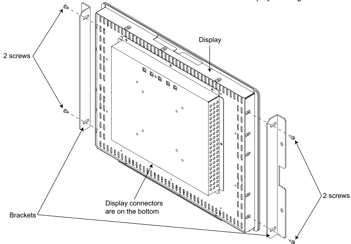
Figure 2 Display Assembly (back view)
