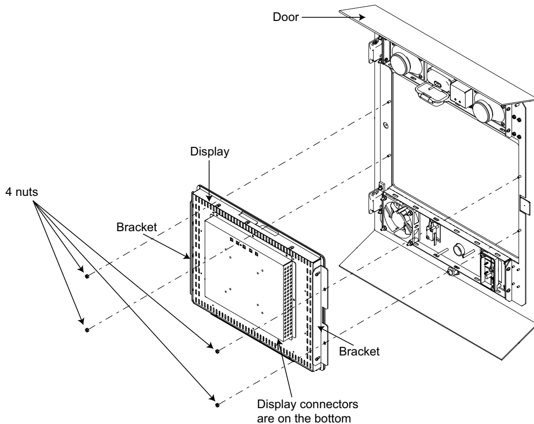
Figure 1 Display on door (back view)
