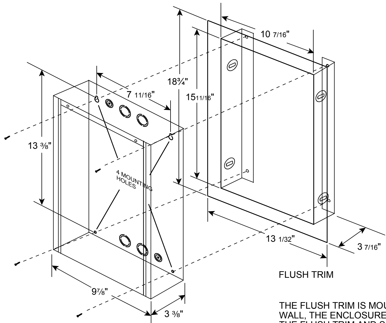
ENCLOSURE
