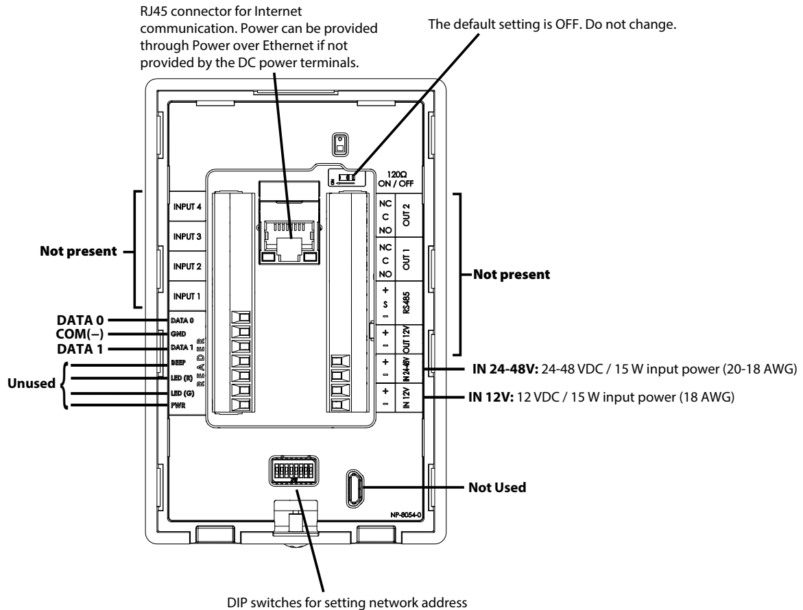
Figure 2. Connections on TX3-IP-WIEGAND
