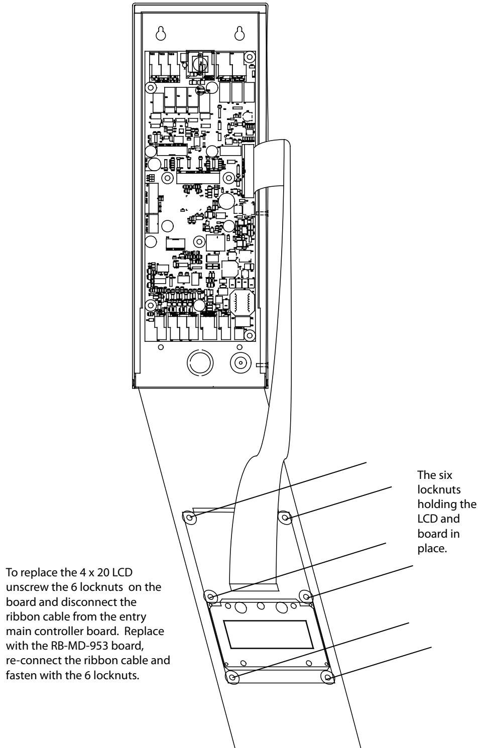
Figure 1: RB-MD-953 Board Replacement
