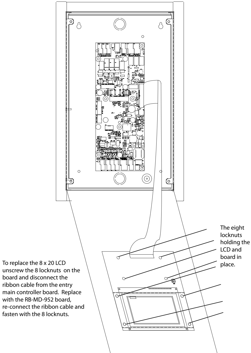
Figure 1: RB-MD-952 Board Replacement
