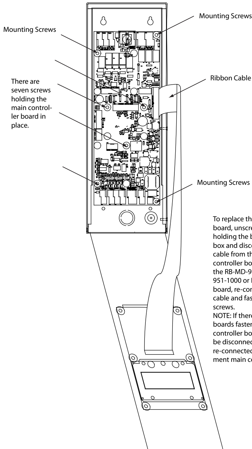
Figure 1: RB-MD-951-200;-1000;-2000 Board Replacement
