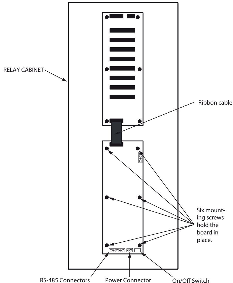
Figure 1 RB-MD-1400-256 TX3-ER-8-B-256 Board Replacement
