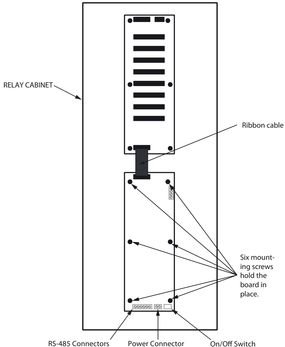
Figure 1: RB-MD-1094 TX3-ER-8-A Board Replacement
