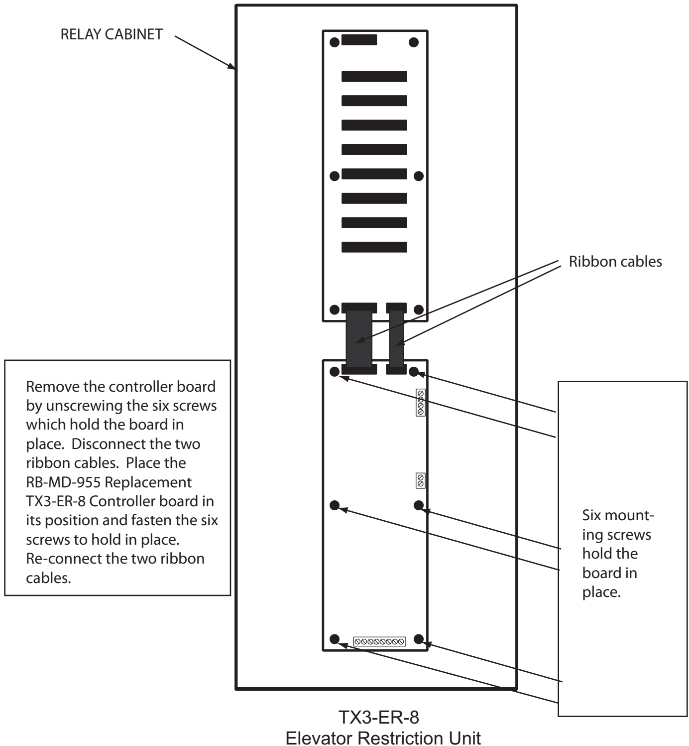
Figure 1: RB-MD-955 TX3-ER-8 Board Replacement
