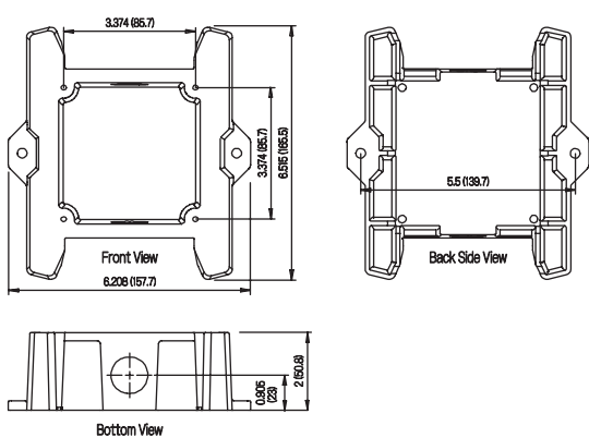
OPTIONAL BBX-5 Outdoor Back Box
