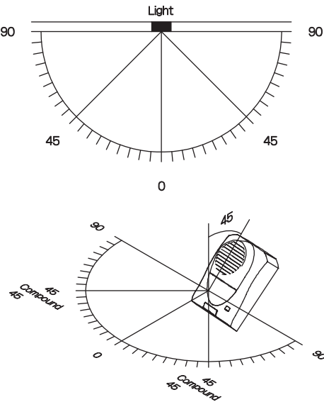
Wall mount horizontal dispersion
